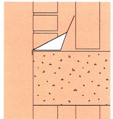
Type G cavitrays used in ringbeam/concrete frame situation. The end upstands terminate against the vertical columns. The protective panoplied lip protects the bedding course.
