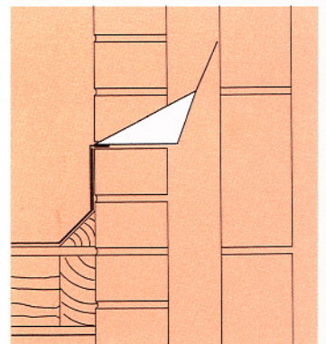
Type G cavitrays with lead attached used at a change of level to ensure the horizontal intersection is correctly damp-proofed and weatherproofed.
