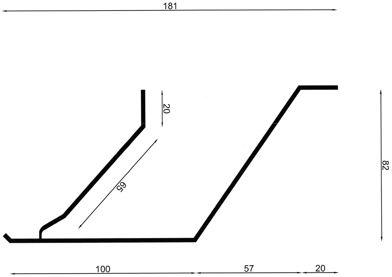
RAV-FL Section
